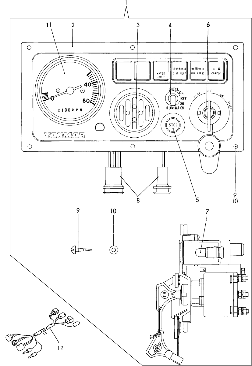
Fig.40 計器盤 (Bタイプ) INSTRUMENT PANEL (B-TYPE)
