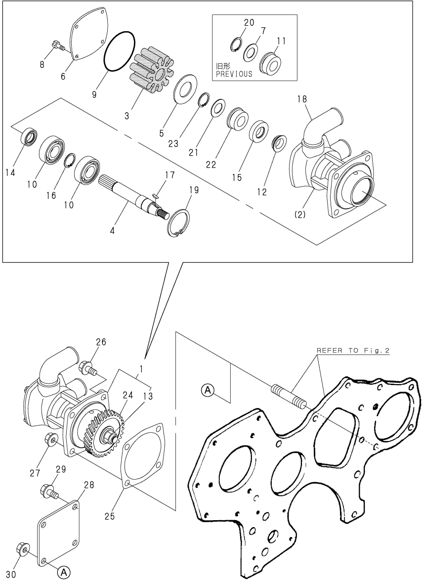
Fig.16 冷却水ポンプ (海水) COOLING SEA WATER PUMP
